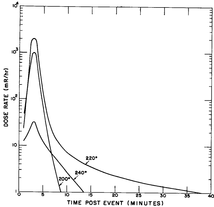
Fig. 24. Ion chamber stations at 8,000 feet.
