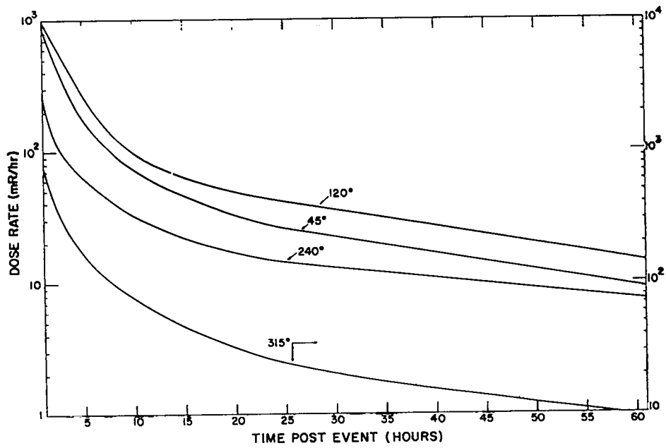
Fig. 25. Ion chamber stations at 500 feet.
