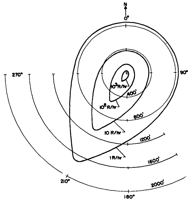
Fig. 29. Isodose rate contours 10 minutes post event.
