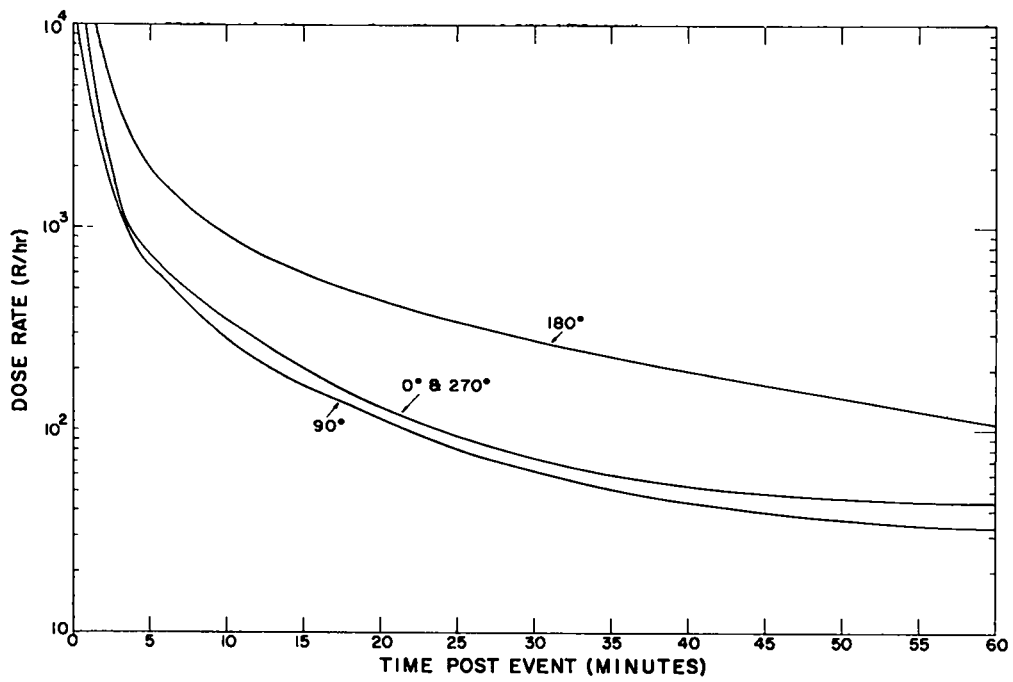
Fig. 16. PV/PM stations at 100 feet.
