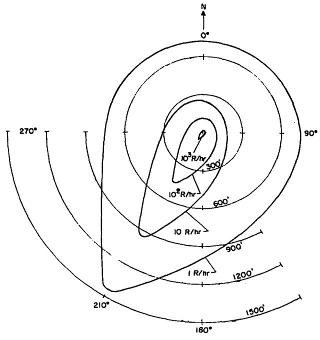
Fig. 30. Isodose rate contours 20 minutes post event.
