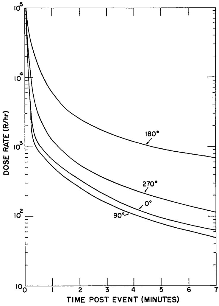
Fig. 14. PV/PM stations at 200 feet.
