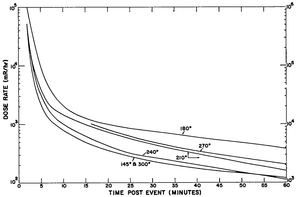
Fig. 21. Ion chamber stations at 1,000 feet.
