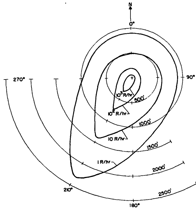
Fig. 28. Isodose rate contours 5 minutes post event.
