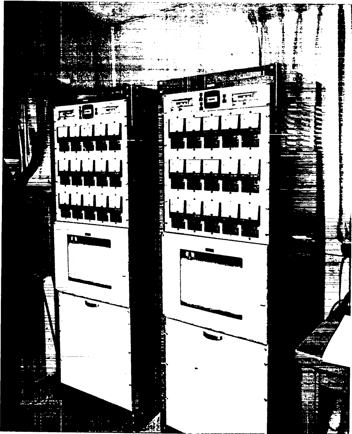
Fig. 9. Ionization chamber readout units.
