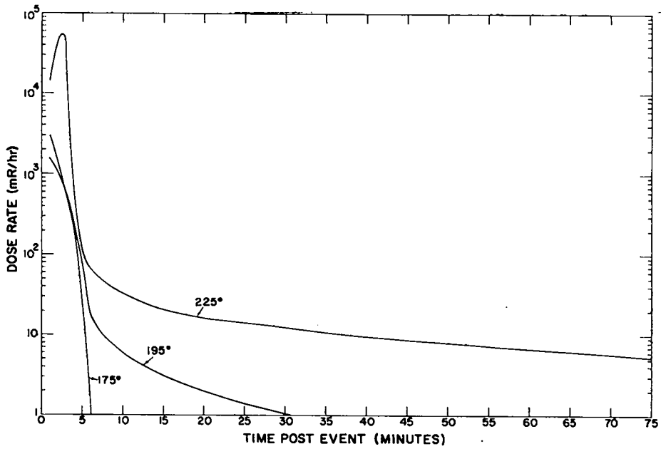
Fig. 23. Ion chamber stations at 4,000 feet.
