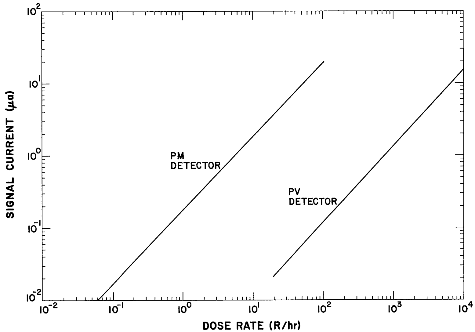
Fig. 7. Response of typical PV and PM detector units.
