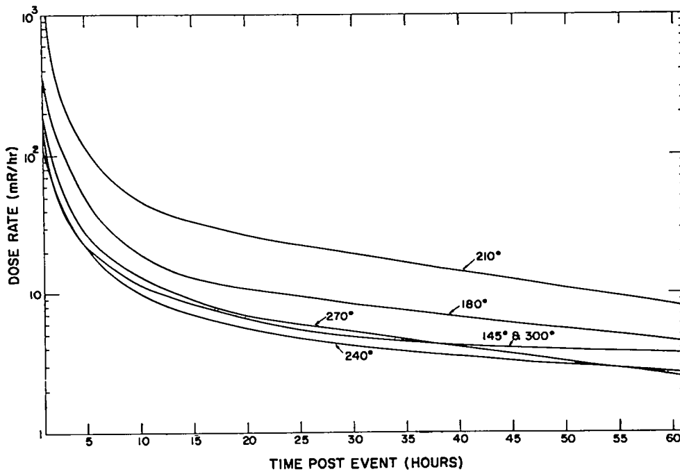
Fig. 26. Ion chamber stations at 1,000 feet.
