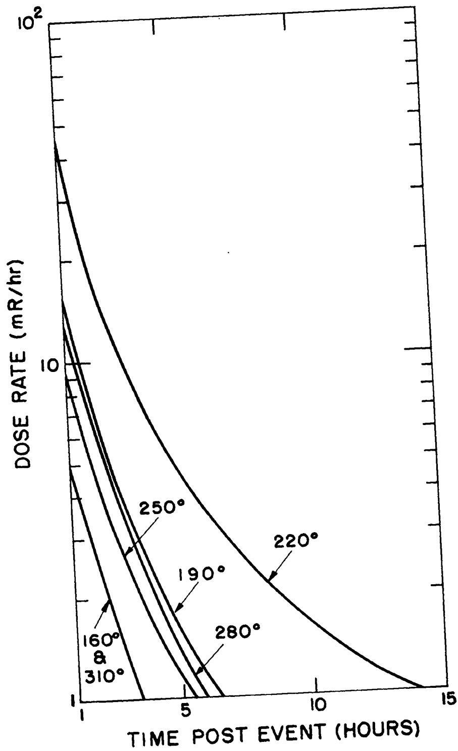
Fig. 27. Ion chamber stations at 2,000 feet.
