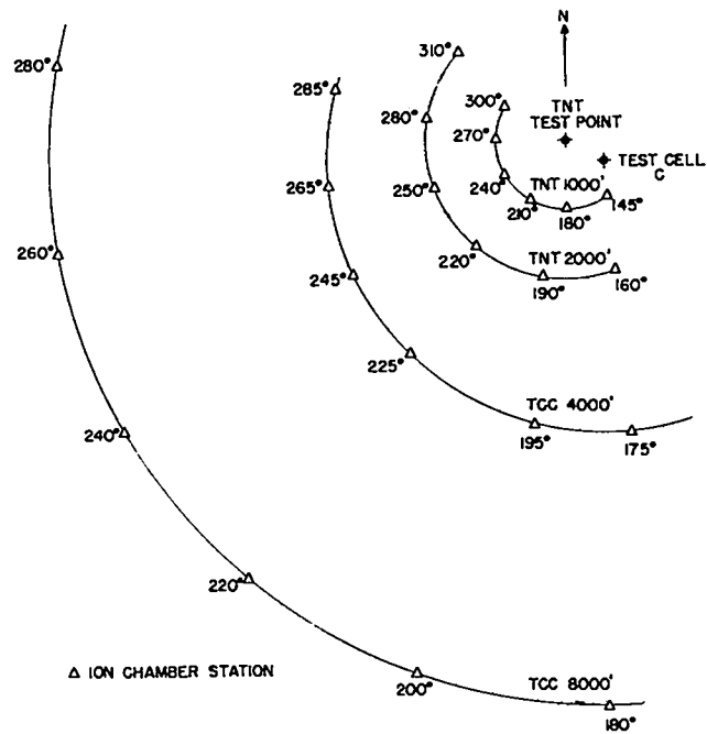
Fig. 11. Location of dose-rate stations, 1,000 to 8,000 feet.
