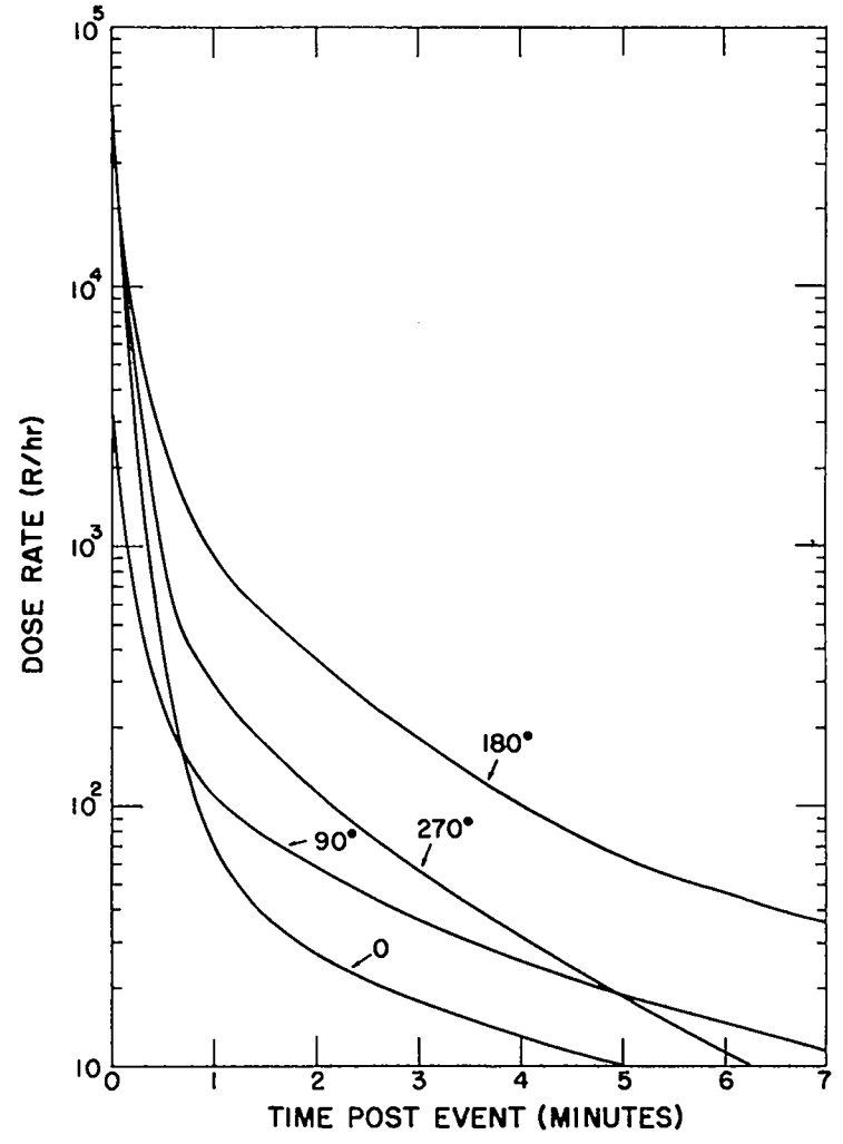
Fig. 15. PV/PM stations at 500 feet.
