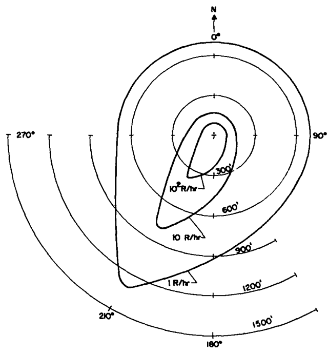
Fig. 31. Isodose rate contours 30 minutes post event.
