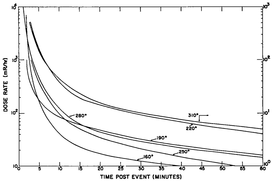
Fig. 22. Ion chamber stations at 2,000 feet.
