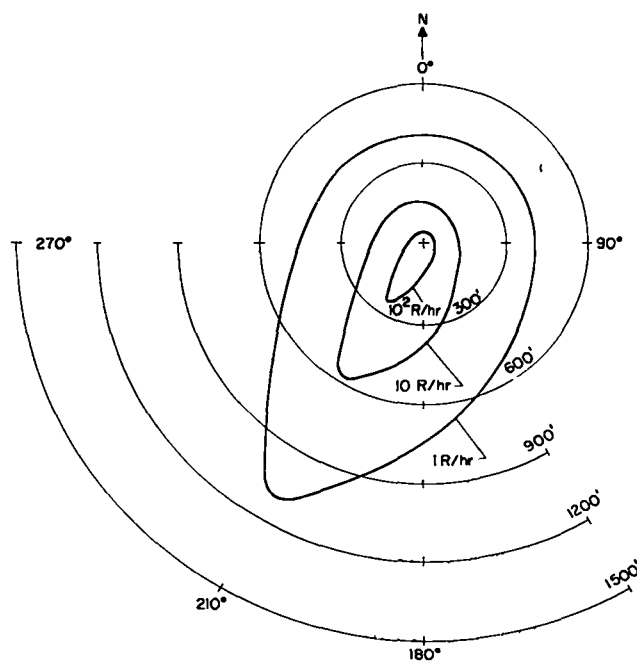
Fig. 32. Isodose rate contours 60 minutes post event.
