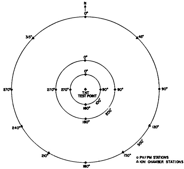
Fig. 10. Location of dose-rate stations, 100 to 500 feet.
