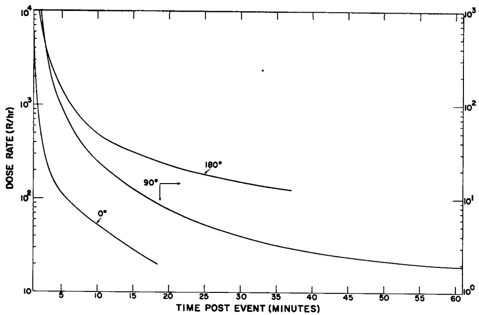
Fig. 17. PV/PM stations at 200 feet.
